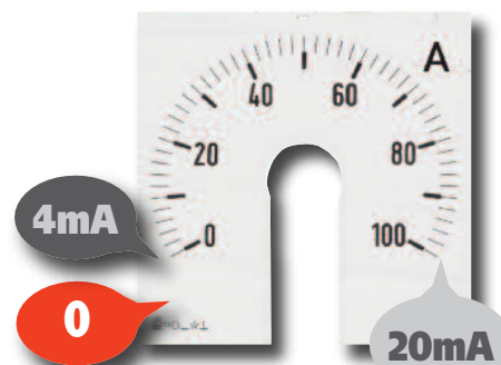
0/4...20mA Soppressione meccanica Mechanically suppressed
