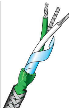
Stainless Steel Braided PFA Twisted with Screen One pair of stranded conductors. PFA insulated. Pair twisted, screened with Mylar aluminium tape and drain wire. PFA sheathed. Stainless steel braided overall.
