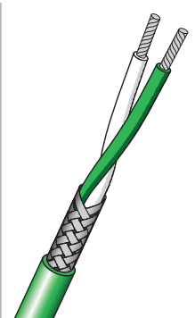
HR PVC Twisted Pair with Tinned Cu Braid One pair of stranded conductors. Cores HR PVC insulated. Pair twisted with tinned copper braid. HR PVC sheathed overall.
